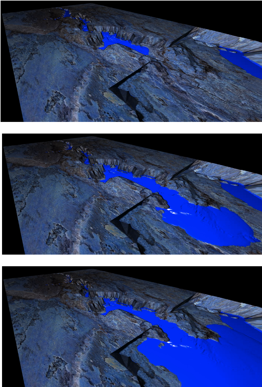
FIGURE 4. Propagation of the Malpasset dam break for different time 1000s, 2000 s and 3000 s.
