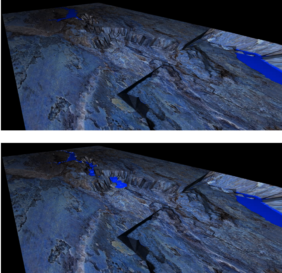
FIGURE 3. Propagation of the Malpas dam break for different time 0 s and 500 s.
