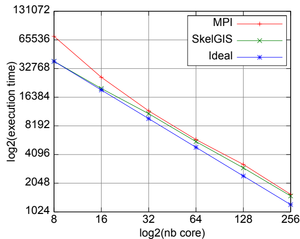
FIGURE 13. Comparison between MPI, SkelGIS and Ideal versions of shallow water equations for 5000 time iterations : Log 2 of execution times
